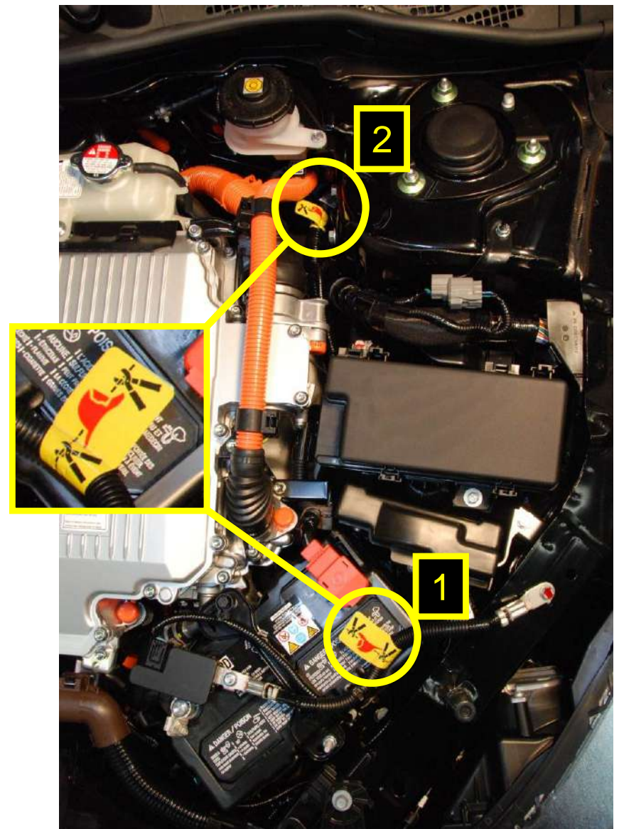
Cut the negative 12V battery cable and then cut the DC to DC Converter cable.
